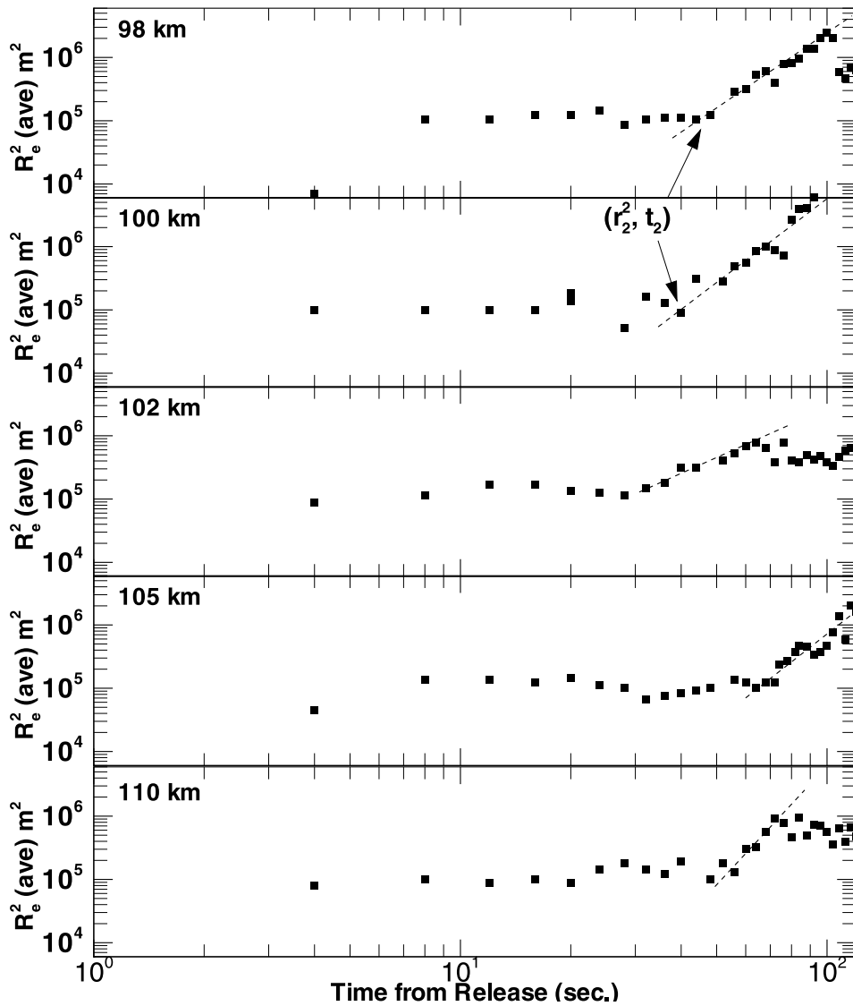
Figure 10. Expansion rates for the altitudes 98, 100, 102, 105, and 110 km.
