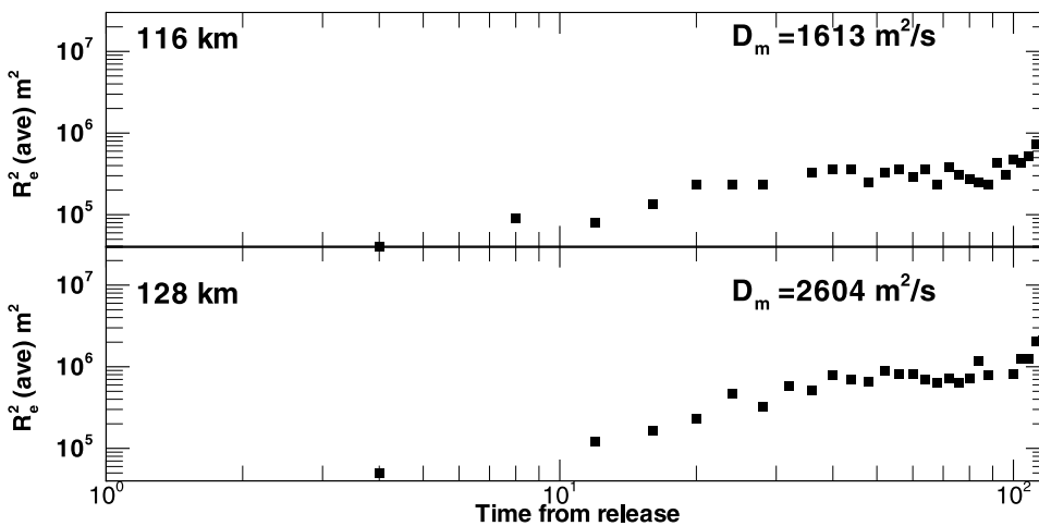
Figure 11. The expansion rates for the altitudes 116 and 128 km are shown from release. Effective radius is defined as the position of the 1/e decrease in intensity from the trail center. The molecular diffusion coefficient as calculated from equation (9) is listed.
