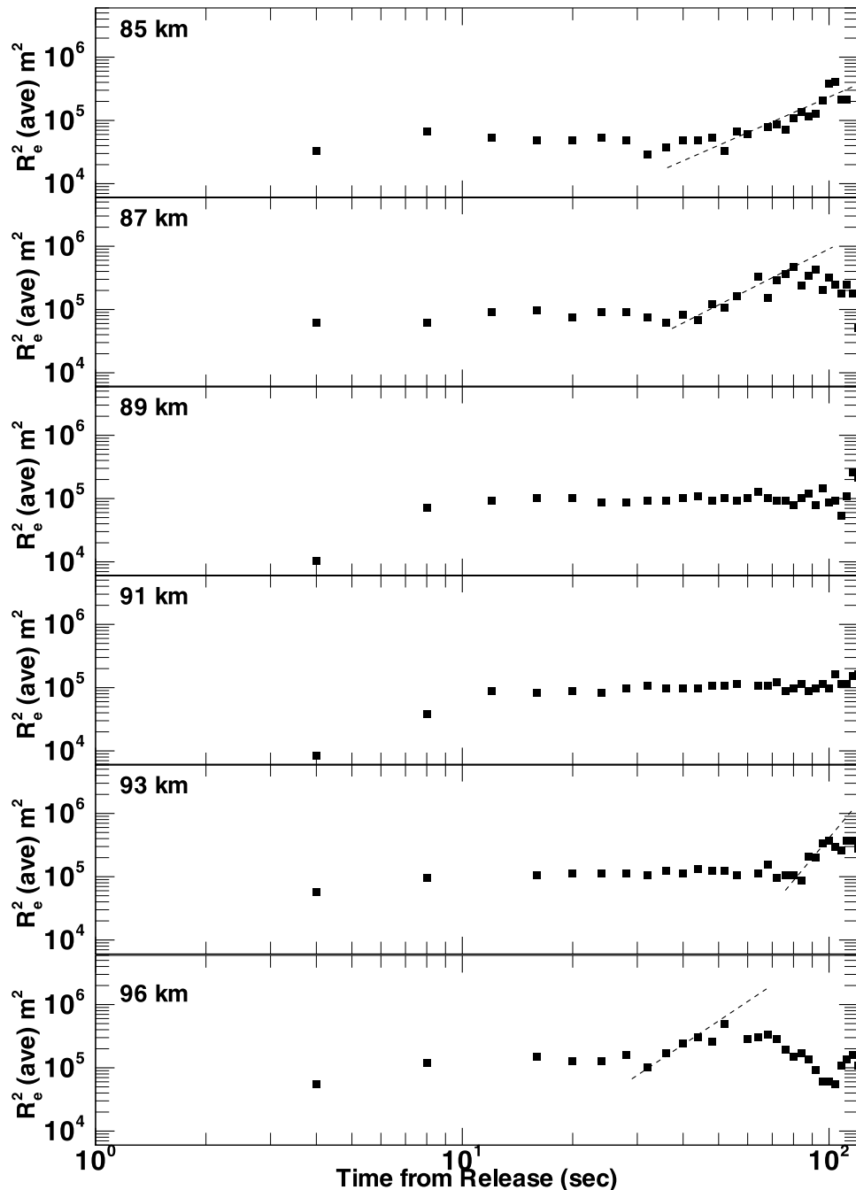
Figure 9. Expansion rates for the altitudes 85, 87, 89, 91, 93, and 96 km. The dashed lines indicate the period when eddy diffusion dominates.
