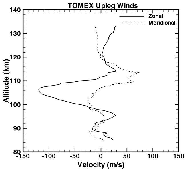
Figure 2. Zonal and meridional winds for the TOMEX upleg release.
