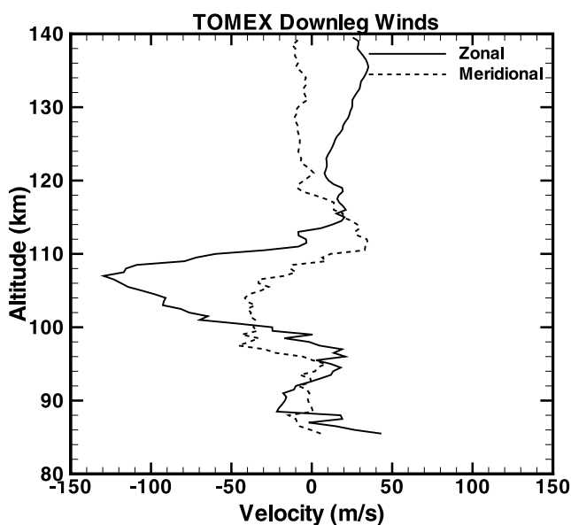
Figure 3. Zonal and meridional winds for the TOMEX downleg release.
